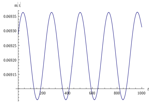
Figure 11: Parameters on the Hopf Bifurcation Boundary
