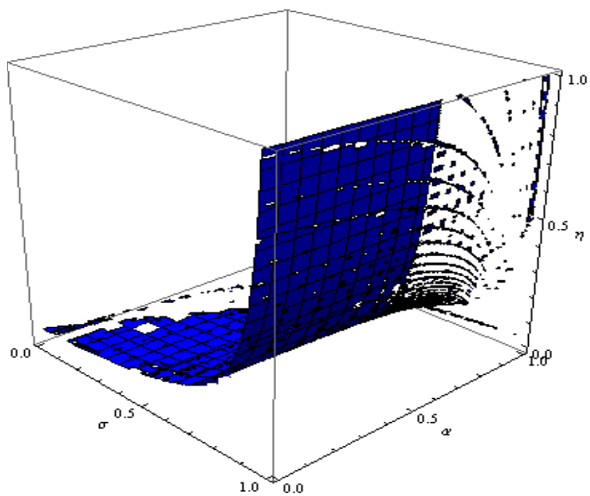
Figure 9: Free Parameters \alpha, \eta, \sigma (Transcritical Bifurcation Boundary)
