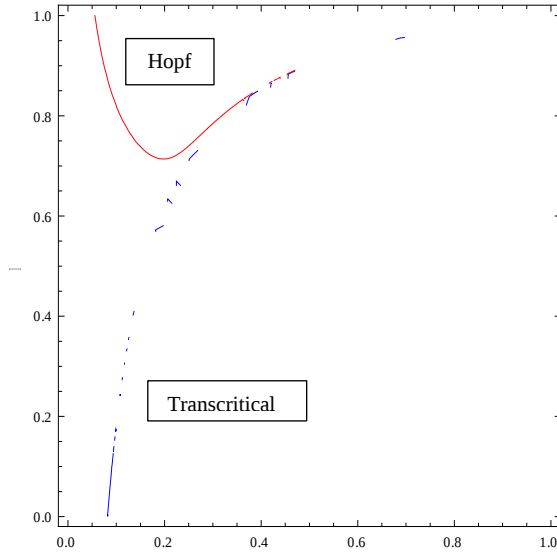
Figure 3: Free Parameters \sigma, \alpha
