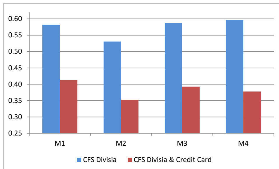
Figure 2: Mean Square Error Comparison (Great Recession)
