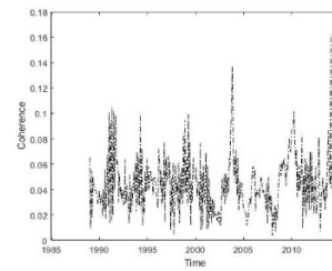
Figure 8.c. The LR coherence function
