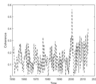
Figure 9.b. The MT coherence function
