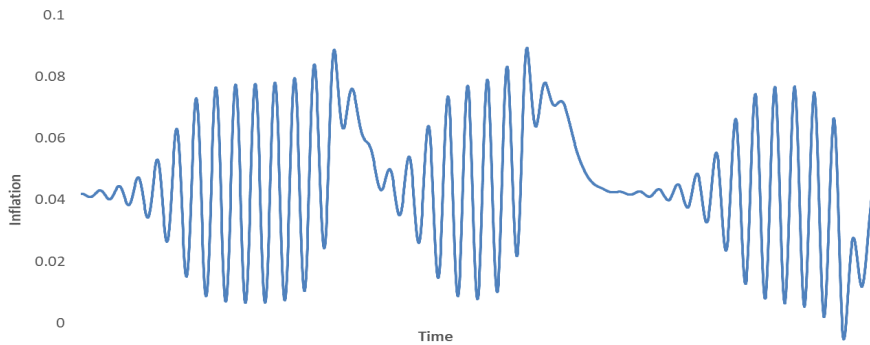
Figure 4. The time profile of the chaotic inflation rate.
